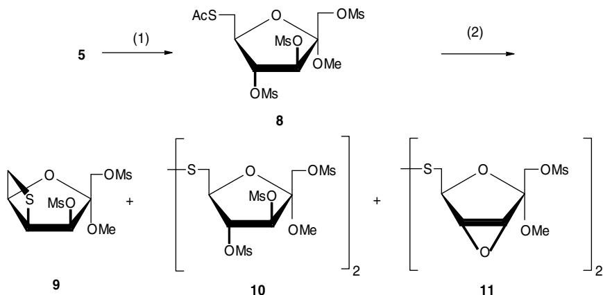
SCHEME 3 (1): MsCl, pyridine; (2): \text{NaHCO}_3 , 2-methoxyethanol.
