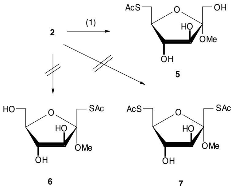
SCHEME 2 (1): AcSH, DIAD, Ph 3 P, THF.
