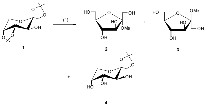
SCHEME 1 (1): HCl, MeOH.
