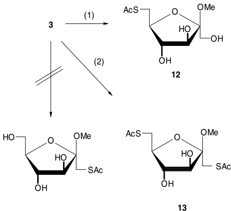
SCHEME 4 (1): 1.27 equiv. AcSH, DIAD, \text{Ph}_3\text{P} , pyridine; (2): 3.0 equiv. AcSH, DIAD, \text{Ph}_3\text{P} , pyridine.
