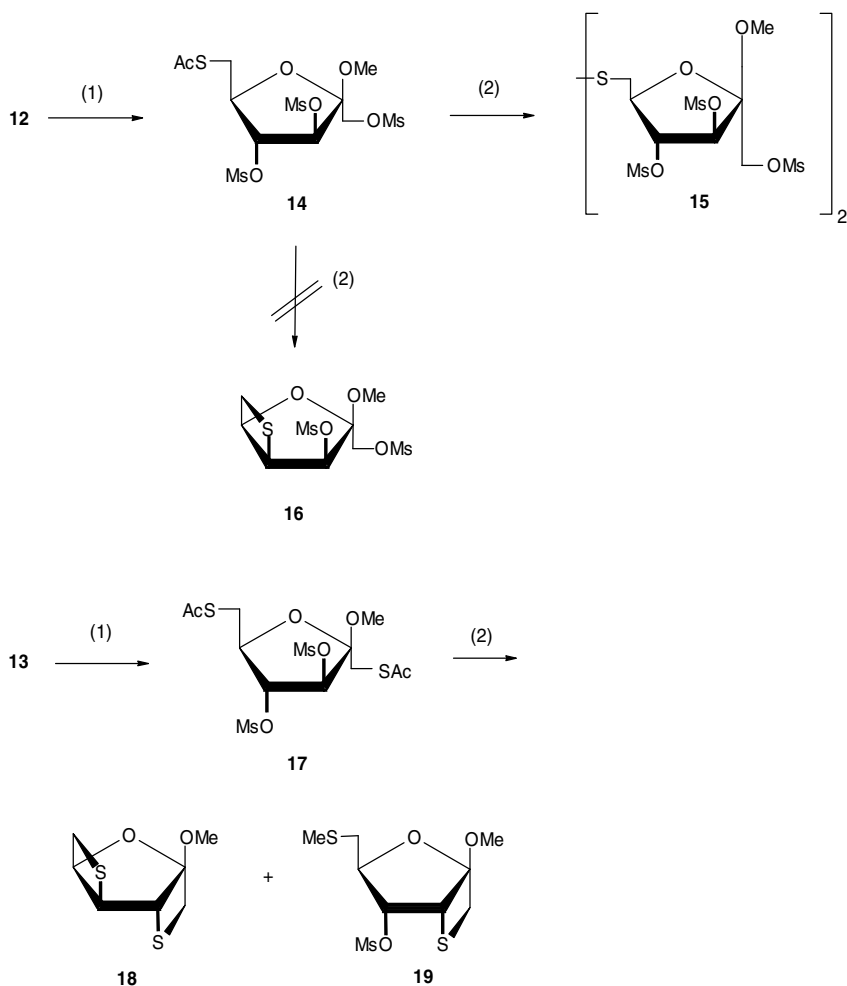
SCHEME 5 (1): MsCl, pyridine (2): NaHCO 3 , 2-methoxyethanol.
